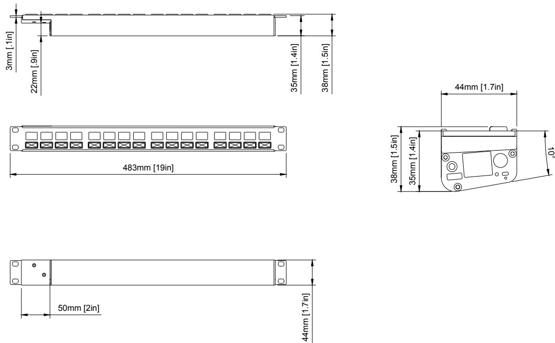
Figure 1: Technical drawing of Frame Shot Uno with key dimensions and layout details.
