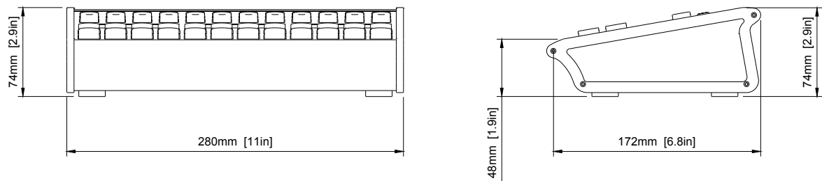
Figure 1: Technical drawing of Master Key 48 with key dimensions and layout details.
