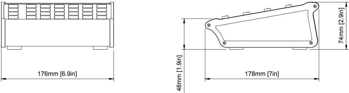
Figure 1: Technical drawing of Quick Shot Pro - Black with key dimensions and layout details.
