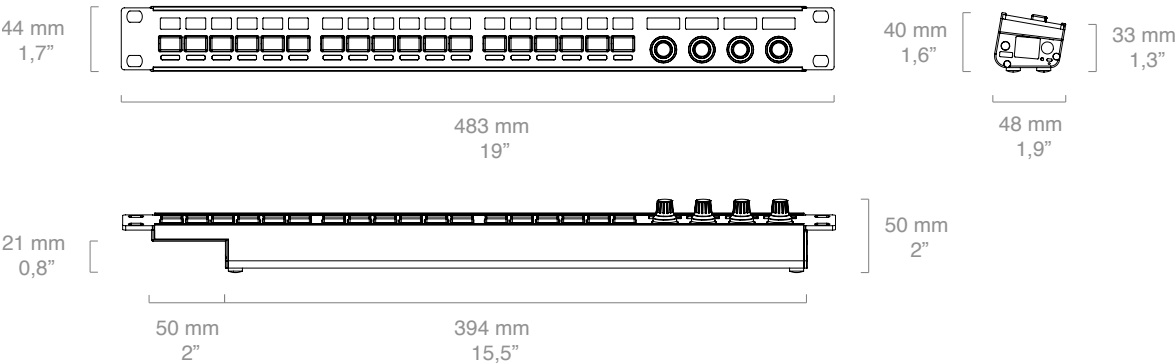
Figure 1: Technical drawing of Rack Control Uno with key dimensions and layout details.
