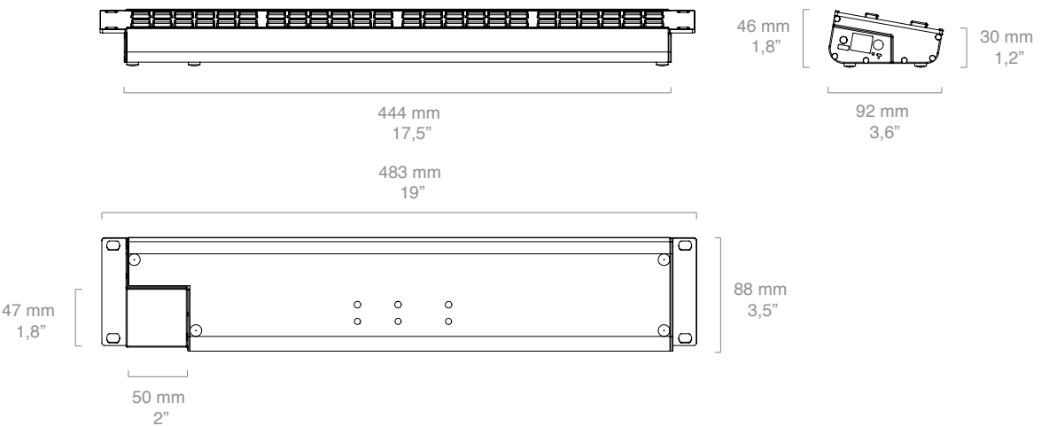
Figure 1: Technical drawing of Rack Fly Duo with key dimensions and layout details.
