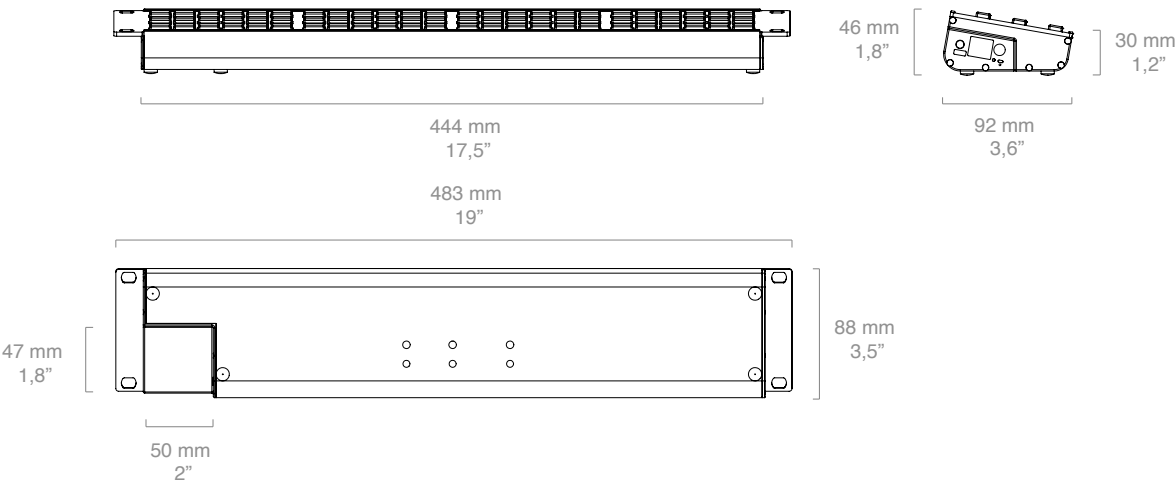
Figure 1: Technical drawing of Rack Fly Trio with key dimensions and layout details.
