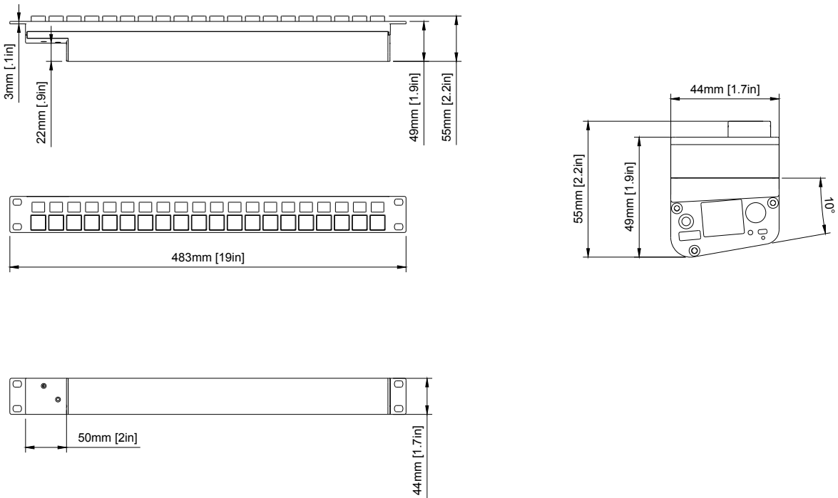
Figure 1: Technical drawing of Rack Pro 1 with key dimensions and layout details.
