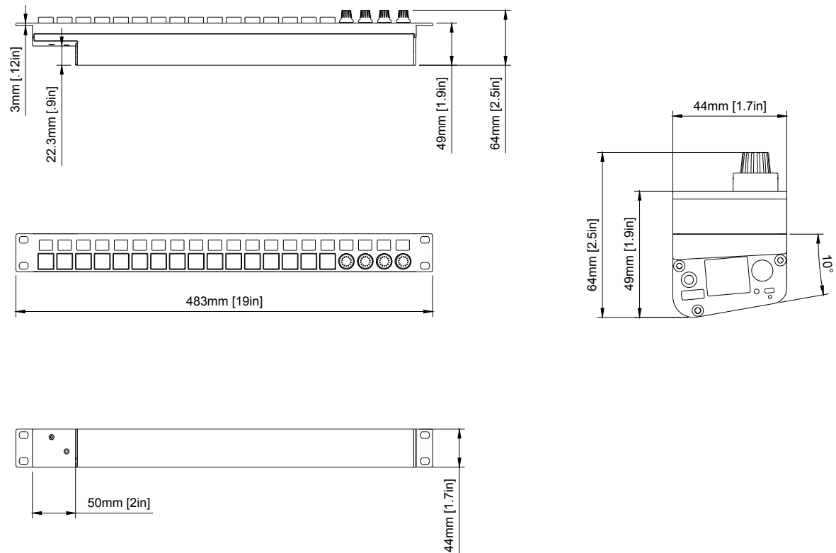
Figure 1: Technical drawing of Rack Pro 3 with key dimensions and layout details.
