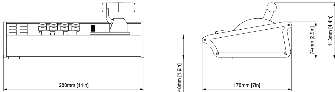
Figure 1: Technical drawing of T-Block Right with key dimensions and layout details.
