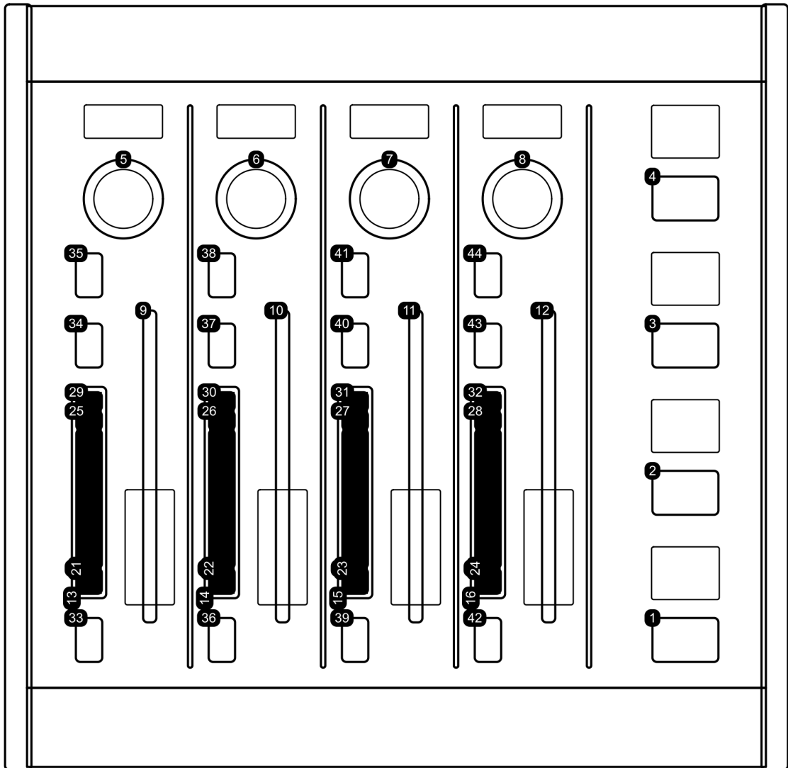
Figure 2: Diagram of hardware components for Wave Board Mini with component IDs (HwC ID)
